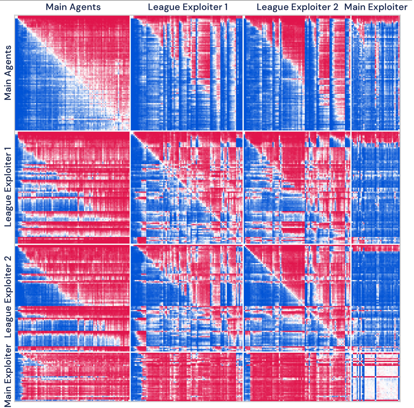
Extended Data Fig. 8 | Payoff matrix (limited to only Protoss versus Protoss games for simplicity) split into agent types of the league. Blue means a row agent wins, red loses, and white draws. The main agents behave transitively: the more recent agents win consistently against older main agents
